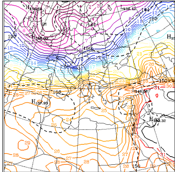
Fig. 5 The air temperature field, at 850 hPa level, on 21-08-99 (12 UTC)
