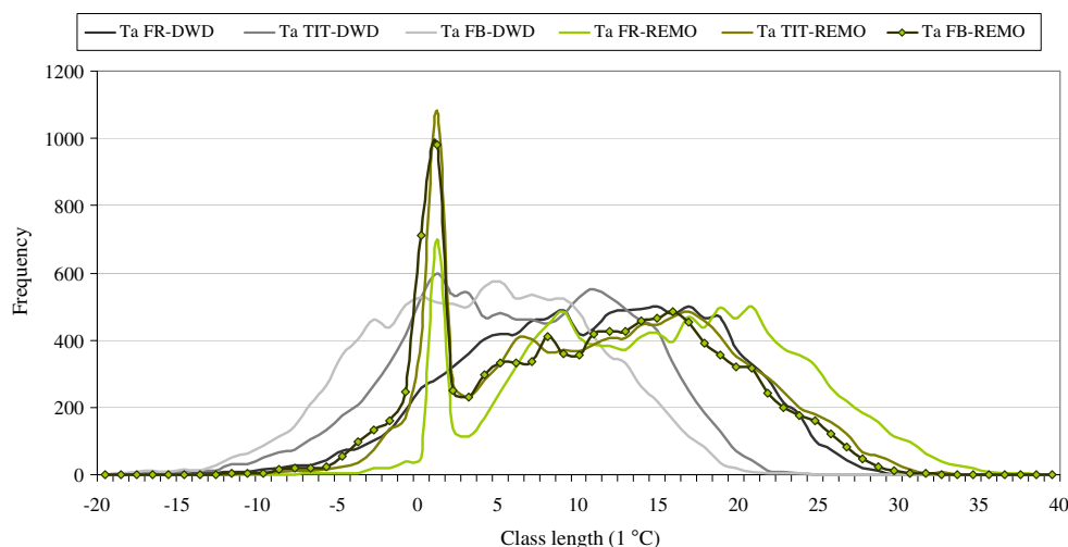
Fig. 2 Frequency distribution of T_a over the time period 1961–1990 based on climate (DWD) and modelled (REMO) data for three stations in the Black Forest: FR Freiburg, TIT Titisee, FB Feldberg
