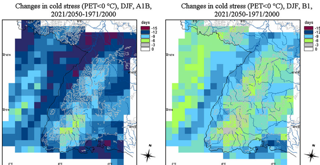
Fig. 4 Changes in winter (DJF) cold stress (PET < 0°C) for the Black Forest region for the period 2021/2050–1971/2000 based on the SRES scenarios A1B (left) and B1 (right)
